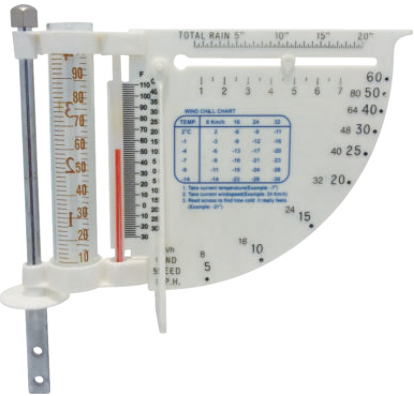
Model:ZLS-136 4-in-1 Weather Station Product size :180*175*58mm Material:PS
