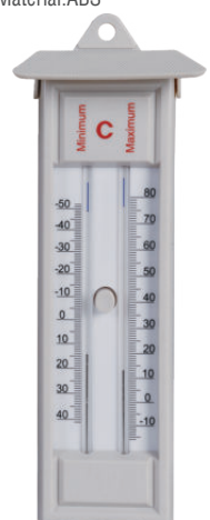
Model:ZL-101 Maximum-Minimum Thermometer Product size :230*80*32mm Material:ABS
