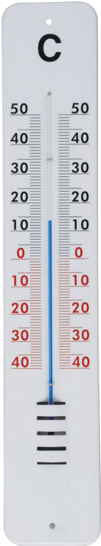
Model:ZL-167 Metal Garden Thermometer Product size :456*80*6mm Material:Iron
