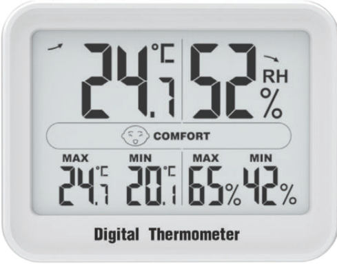
Model:SH-019 Digital Thermometer Product size : 130*101*25mm Material:ABS
