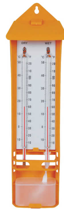
Model:ZL-084 Psychrometer Product size :330*90*45mm Material:PS
