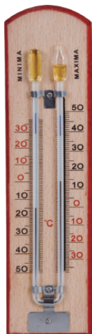
Model:ZL-112 Maximum-Minimum Thermometer Product size :216*56*16mm Material:WOOD
