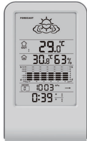
Model:SH-075 Digital Thermometer Product size : 110*77*41mm Material:ABS Transmitter : SH-074T
