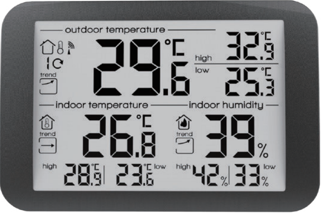
Model:SH-8045C Digital Thermometer Product size : 138.5*92*23mm Material:ABS Transmitter : SH-006T
