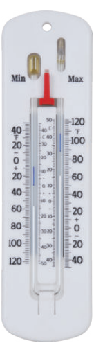
Model:ZL-106 Maximum-Minimum Thermometer Product size : 230*65*15mm Material:ABS
