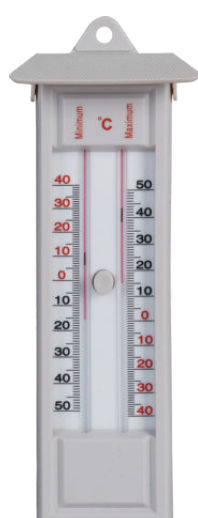
Model:ZL-004 Maximum-Minimum Thermometer Product size :230*80*32mm Material:ABS
