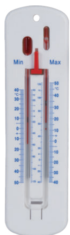
Model:ZL-010 Maximum-Minimum Thermometer Product size :238*65*16mm Material:ABS
